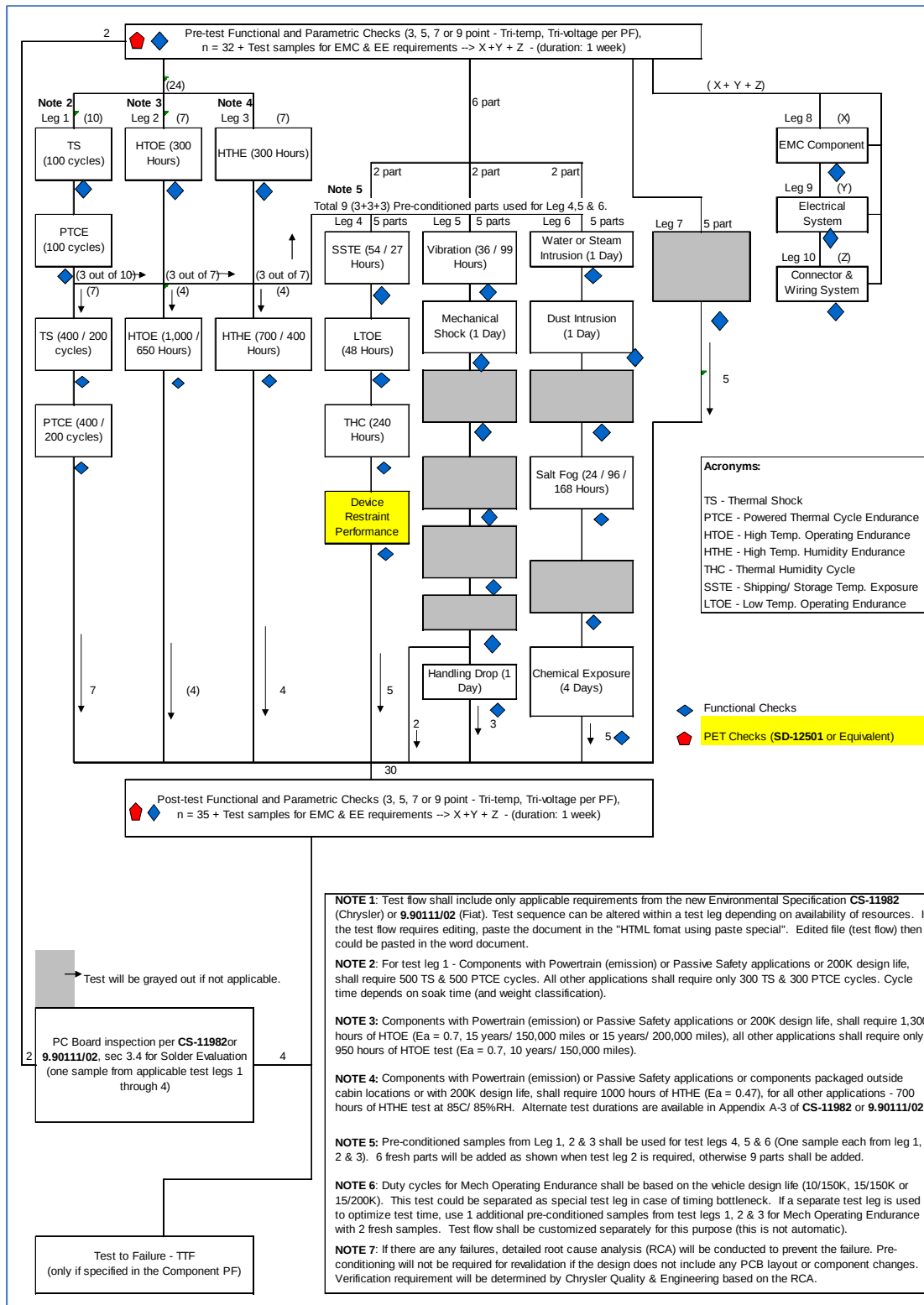
FIGURE A-1: TEST FLOW SEQUENCE FOR EE COMPONENT VALIDATION
